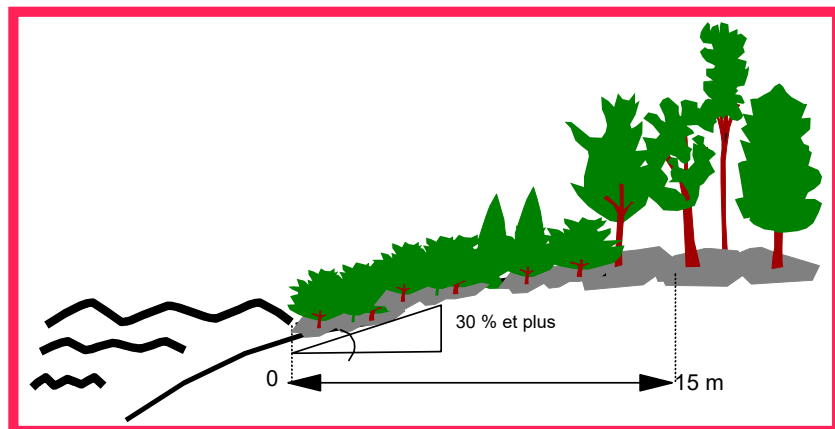
Figure 13.1c : Rive de 15 m (cas no1)
